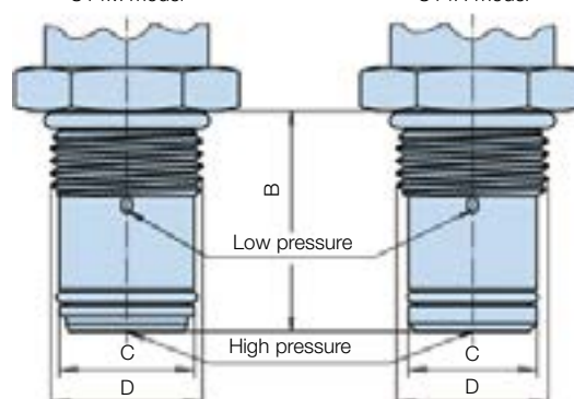
U14M model
