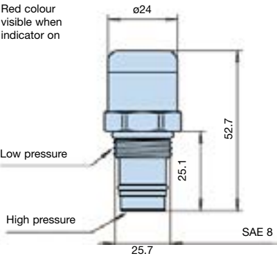
FMUM3 Visual Auto Reset Operation
