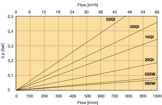
DF65 elements
