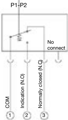
Contact configuration Electrical Indicator Type T1
