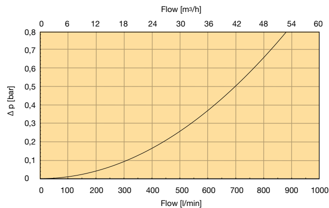
DF65 housing
